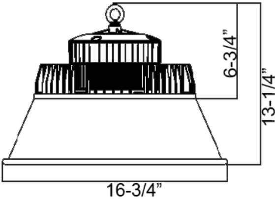
71515 90° Aluminum Reflector
